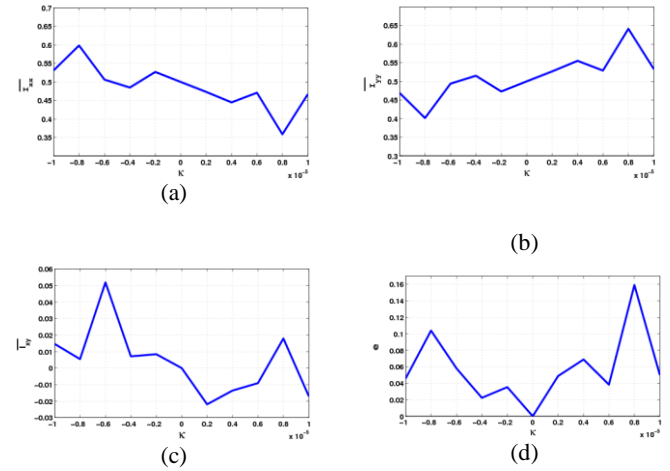
Figure 3: Effect of lens distortion on means of local shading measures: (a) \overline{I_{xx}} , (b) \overline{I_{yy}} , (c) \overline{I_{xy}} , (d) Error \varepsilon_\kappa versus \kappa .
