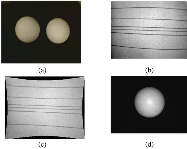
Figure 7: Lens distortion calibration: (a) Calibration image of two balls, (b) Image of straight lines on paper, (c) Undistorted lines image, (d) Another calibration image of one ball.
