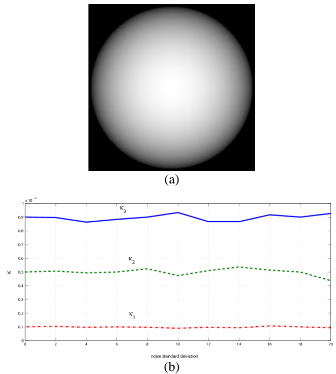
Figure 4: Proposed method performance versus noise: (a) Input synthetic sphere image. (b) The estimated lens distortion coefficient \kappa versus noise standard deviation for 3 ground truth values ( 1 \times 10^{-6} , 5 \times 10^{-6} , and 9 \times 10^{-6} ).
