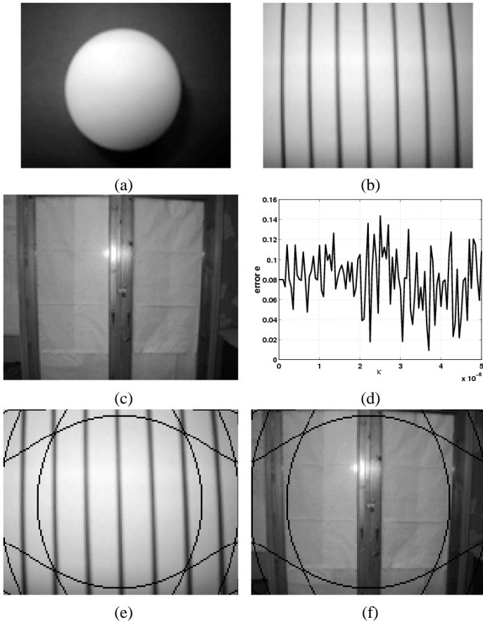
Figure 6: Lens distortion calibration: (a) Calibration image, (b) Image of straight lines on paper, (c) A real scene, (d) \epsilon_x versus \kappa , (e) Undistorted lines image, (f) Undistorted real scene.
