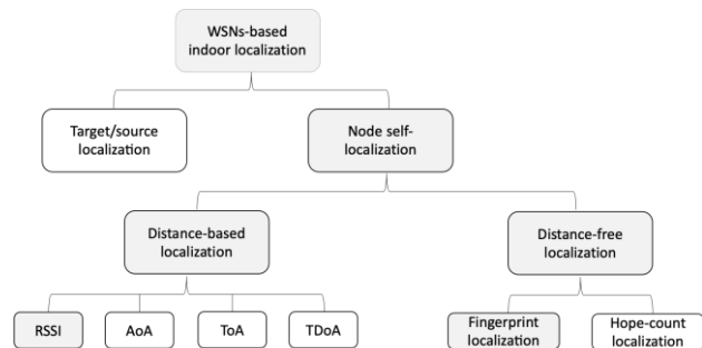
Figure 1. Taxonomy of WSN-based indoor localization[19]
