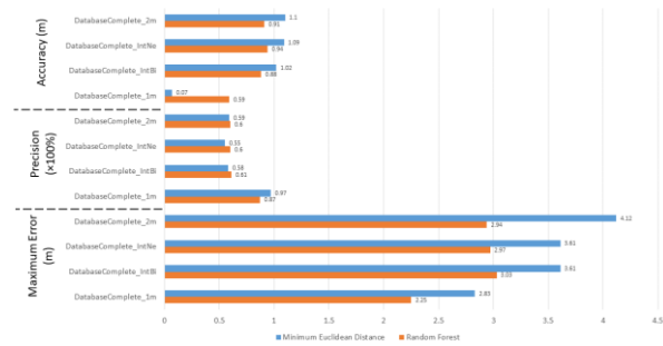
Figure 19. The pattern matching algorithm performance in Scenario 3
