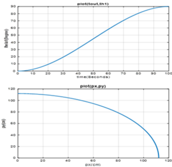
Figure 15. Trajectory plot when \theta_{f1}=0, \theta_f1=90, \theta_f2=0, \theta_f2=0
