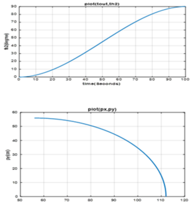
Figure 16. Trajectory plot when \theta_{f1}=0, \theta_f1=0, \theta_f2=0, \theta_f2=90
