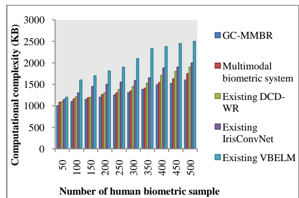
Figure 5 (b) Comparison performances of computational complexity using Biosecure Dataset
