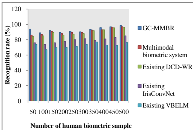
Figure 6 (b) Comparison performances of recognition rate using Biosecure Dataset
