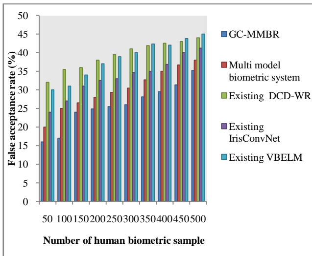
Figure 8 (b) Comparison performances of false acceptance rate using Biosecure Dataset
