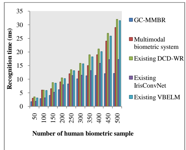
Figure 7 (a) Comparison performances of recognition time using CASIA Biometric Ideal Test Dataset
