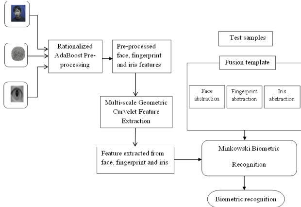
Figure 1 Geometric Curvelet and Minkowski Multimodal Biometric Recognition (GC-MMBR) Block diagram
