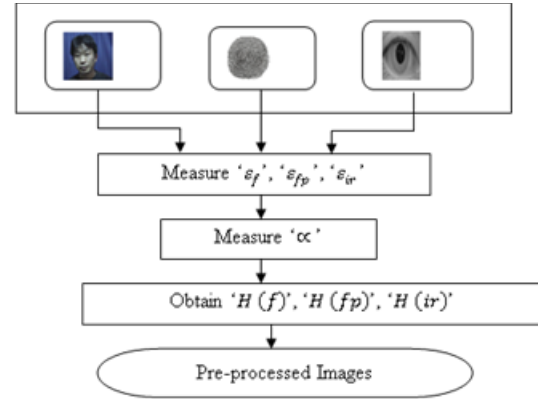
Figure 2. Flow diagram of Rationalized AdaBoost Pre-processing model
