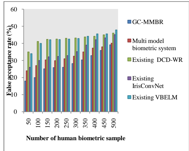
Figure 8 (a) Comparison performances of false acceptance rate using CASIA Biometric Ideal Test Dataset
