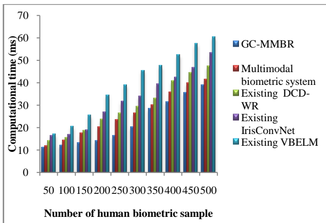
Figure 4 (b) Comparison performances of computational time using Biosecure Dataset
