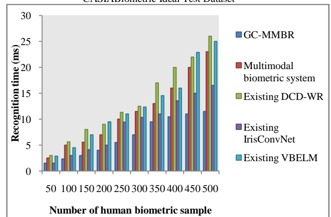
Figure 7 (b) Comparison performances of recognition time using Biosecure Dataset
