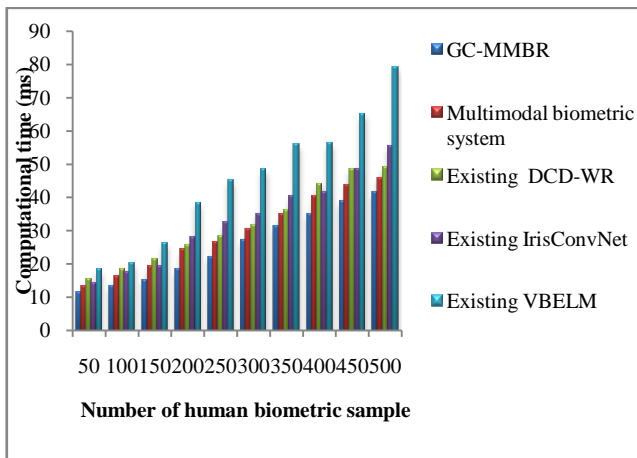
Figure 4 (a) Comparison performances of computational time using CASIA Biometric Ideal Test Dataset
