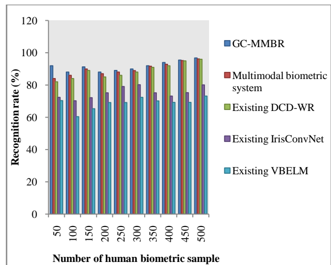
Figure 6 (a) Comparison performances of recognition rate using CASIABiometric Ideal Test Dataset
