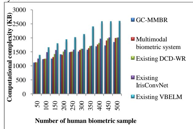
Figure 5 (a) Comparison performances of computational complexity using CASIA Biometric Ideal Test Dataset
