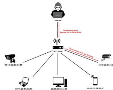
Figure 3. Directed De-authentication Attack
