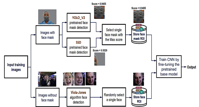
Figure 1. Block diagram of the proposed face mask detector architecture
