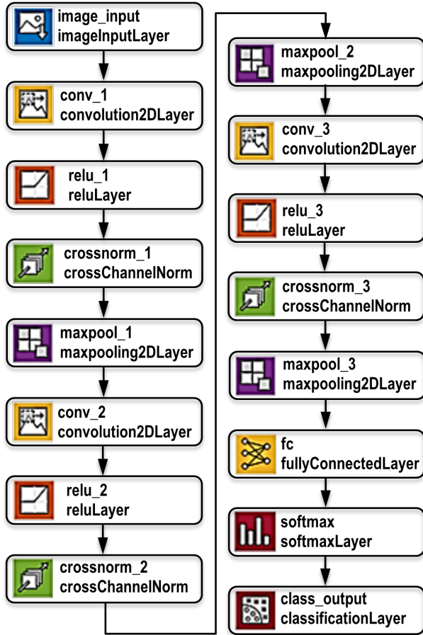
Figure 4. Proposed CNN base model
