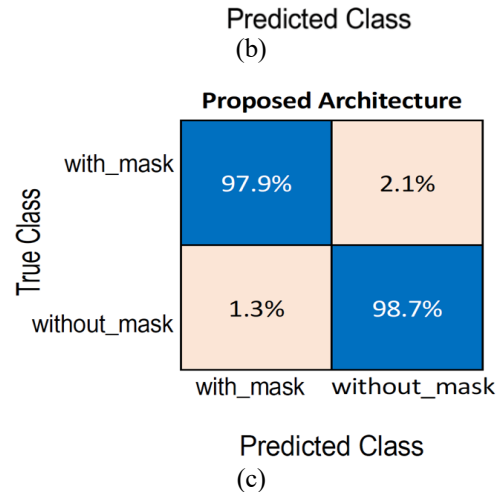
Figure 5. Confusion matrix for (a) the base model, (b) AlexNet, and (c) proposed architecture
