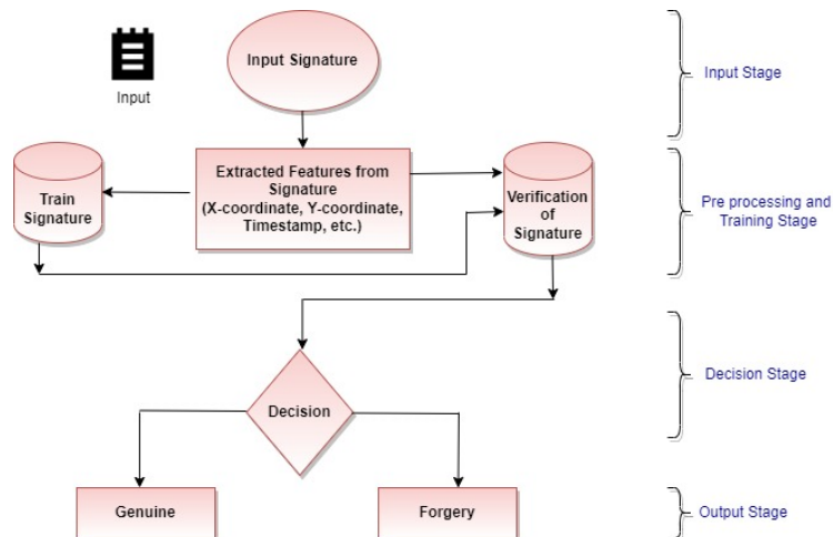
Figure 1. The proposed signature verification methodology
