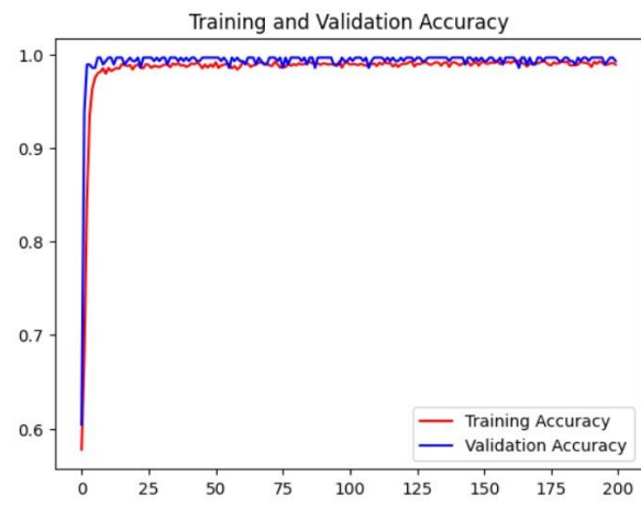
Fig 11. Training and Validation Accuracy
