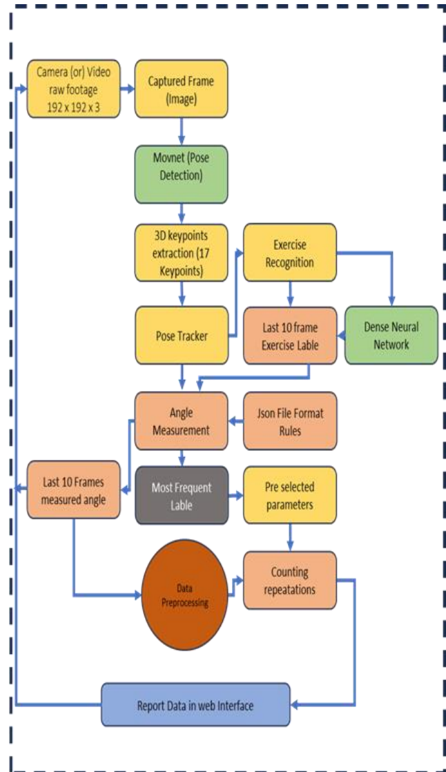
Fig 1. Schematic of the suggested system in blocks
