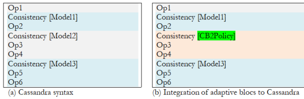
Figure 2. Consistent blocs with Cassandra
