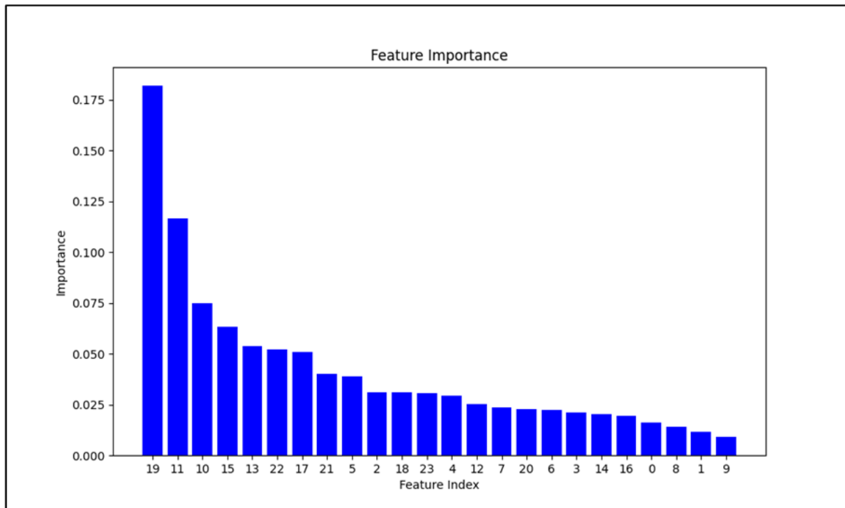
Figure 4 The Sorting of features depending on importance using RF
