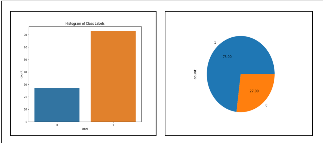
Figure 3 The histogram of class label for dataset
