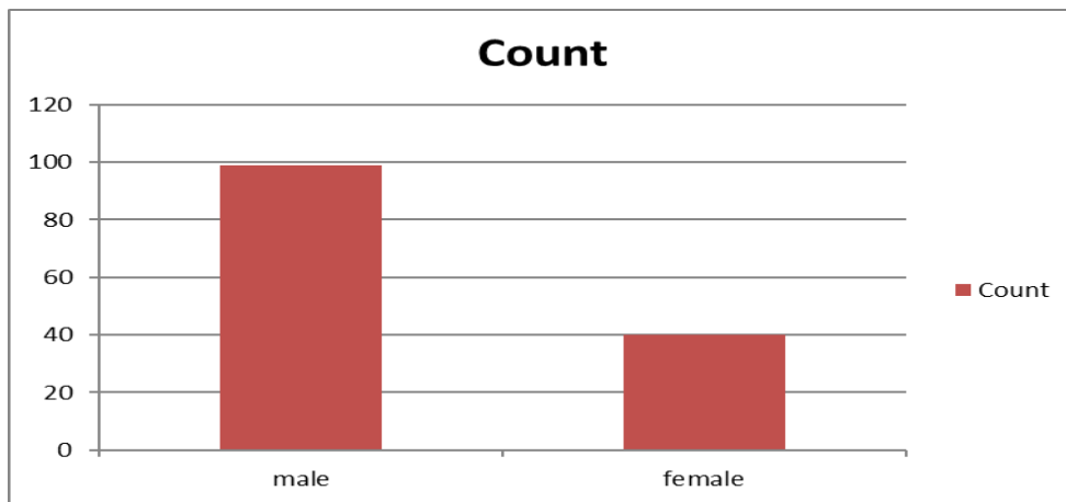
Figure 2 The histogram of male and female counting
