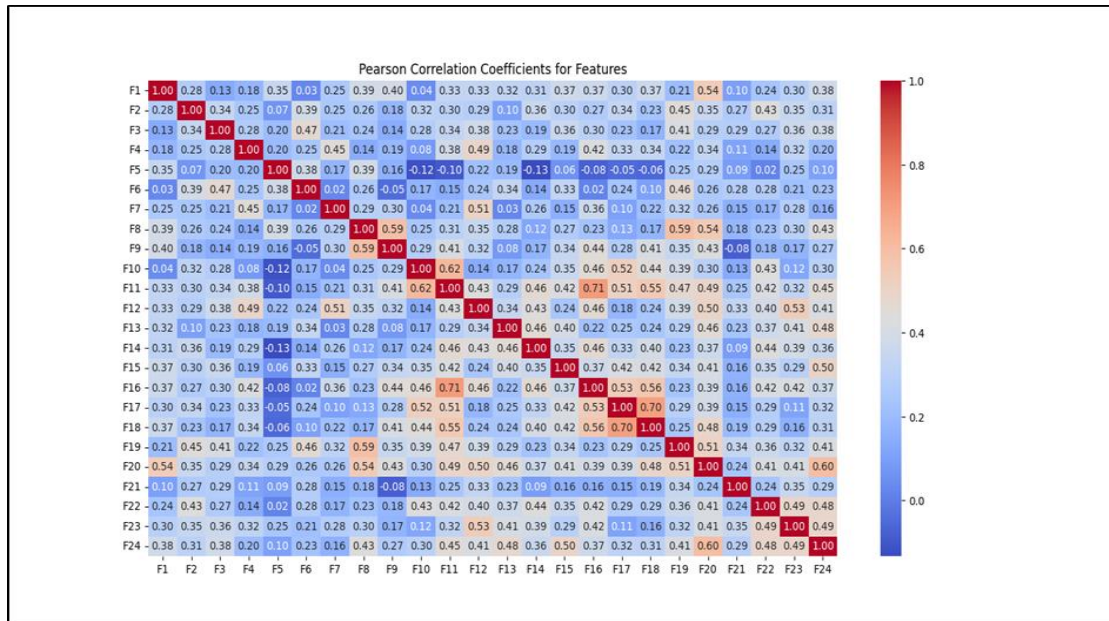
Figure 5 The Person correlation between features
