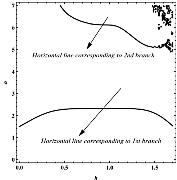
Figure 1 Plot \alpha as a function of h at m = 5 in (3.22) of Bratu's problem (3.16).
