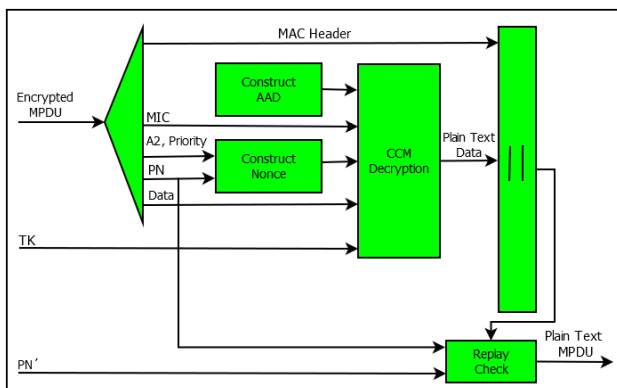
Figure 7. (b) Decryption scheme of MPDU
