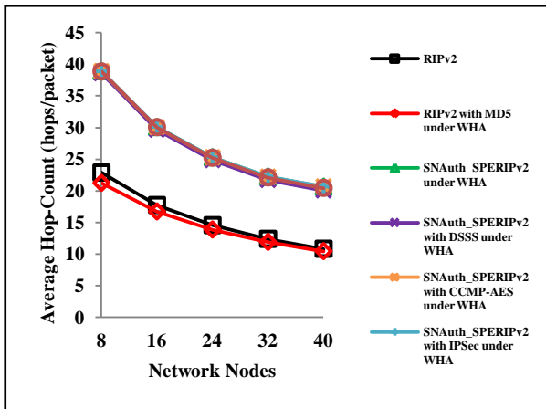
Figure 10(g) Average hop-count versus number of network nodes
