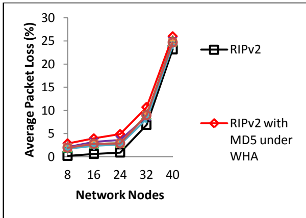
Figure 10 (c) Average packet loss versus number of network nodes
