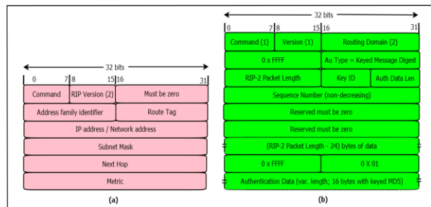
Figure 4. RIP v2 message format (a) with a plain text password (b) keyed MD5
