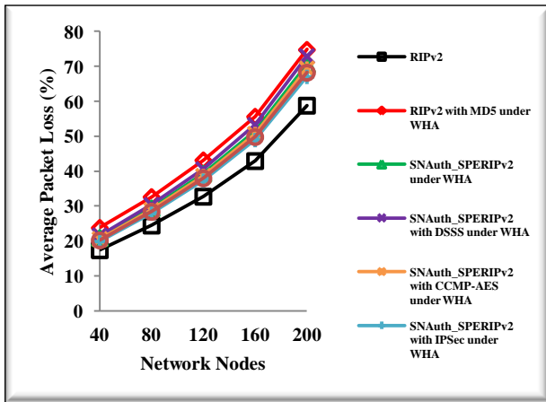
Figure11 (c) Average packet loss versus number of network nodes
