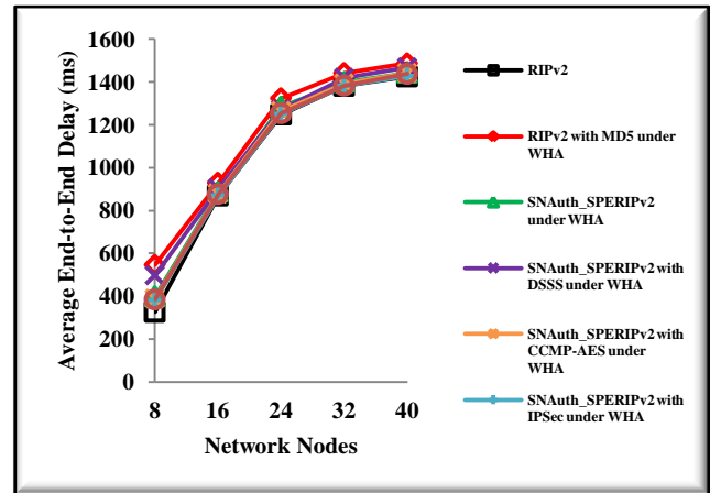
Figure 10(e) Average end-to-end delay versus number of network nodes
