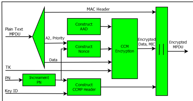
Figure 7. (a) Encryption scheme of MPDU
