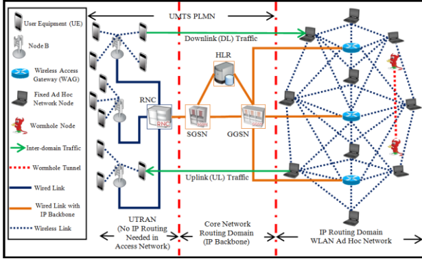
Figure 9. The Integrated UMTS and WLAN Ad Hoc network with WHA adversary
