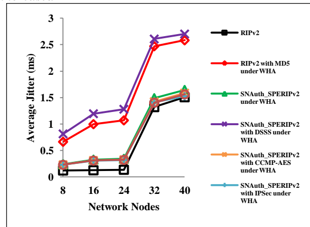
Figure 10(f) Average jitter versus number of network nodes
