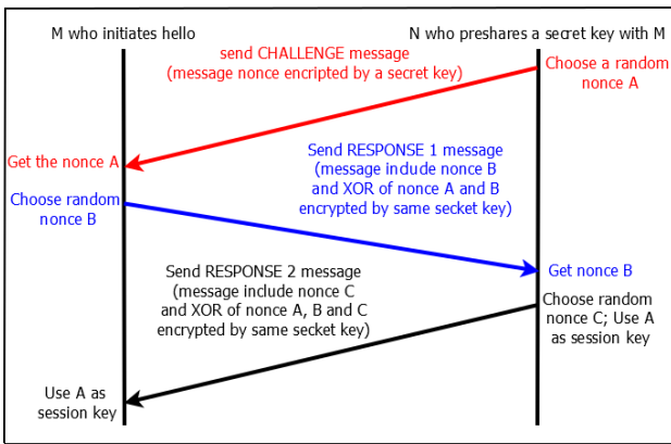
Figure 2. Pair-wise shared secret variant of SNAuth
