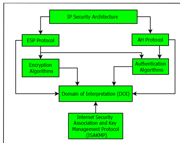
Figure 8. IPSec protocol architecture
