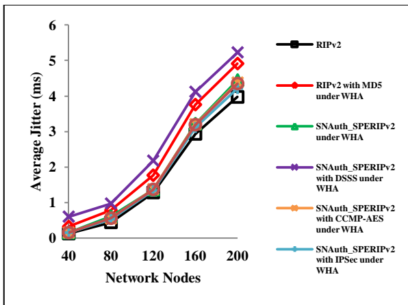
Figure11(f) Average jitter versus number of network nodes
