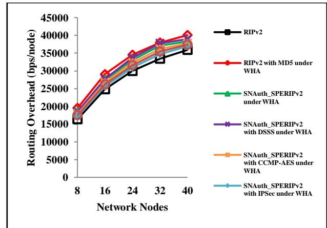
Figure 10(b) Average routing overhead versus number of network nodes
