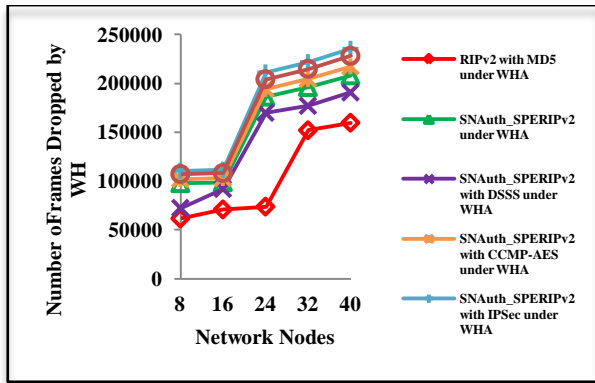
Figure 10(a) Number of frames dropped by WH versus number of network nodes
