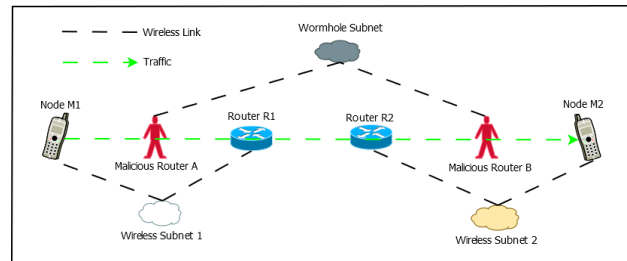
Figure 1. WHA adversary under transparent mode
