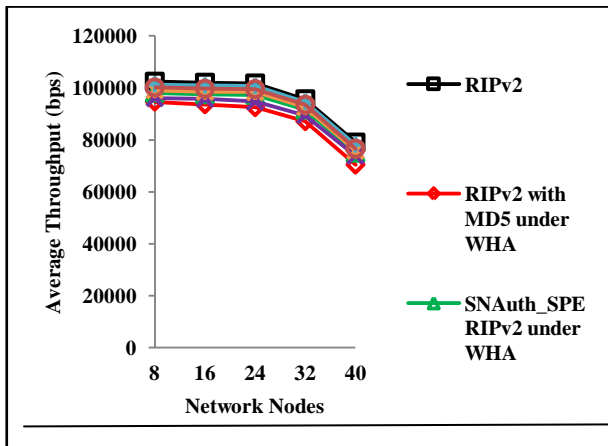
Figure 10(d) Average throughput versus number of network nodes
