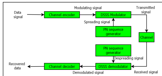
Figure 6. DSSS system model
