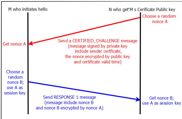
Figure 3. SNAuth variant based on certification
