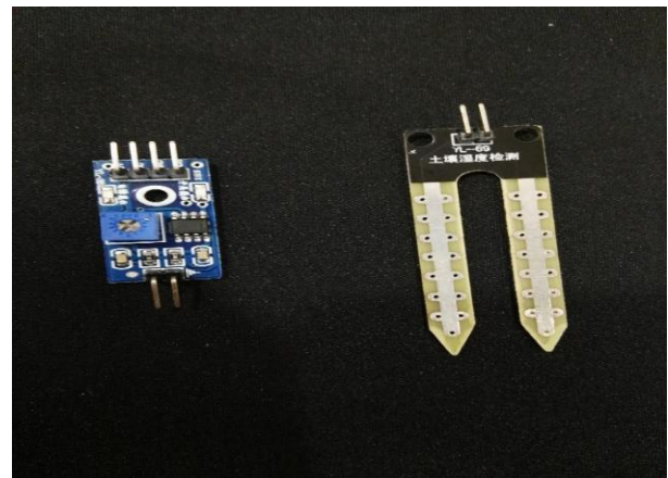
Figure.3. Moisture sensor YL-69.
