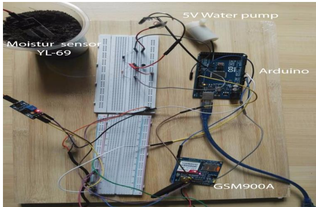
Figure 3. complete hardware circuit of the system.
