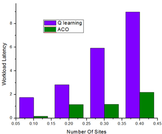
Figure 9. Workload latency
