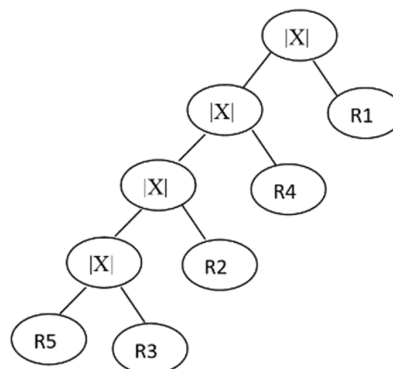
Figure 2. Left-Deep tree (Join Tree Q1)
