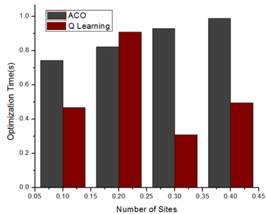
Figure 7. Optimization time
