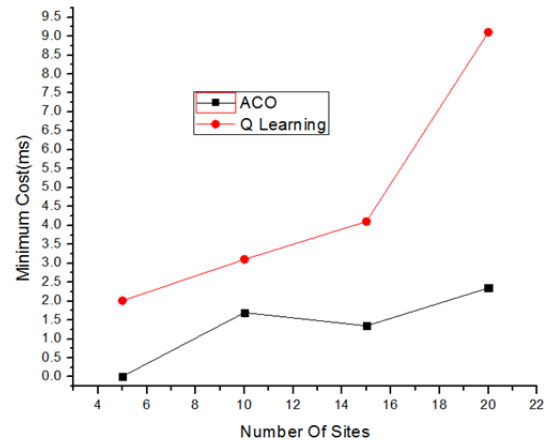
Figure 8. Minimum cost
