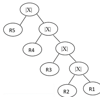
Figure 4. Right Deep Tree (Join Tree Q2)
