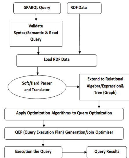
Figure 1. Complete process of query optimization
