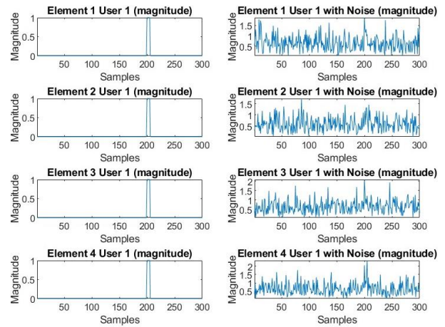
Fig. 4. Noise Signal added to Users1
