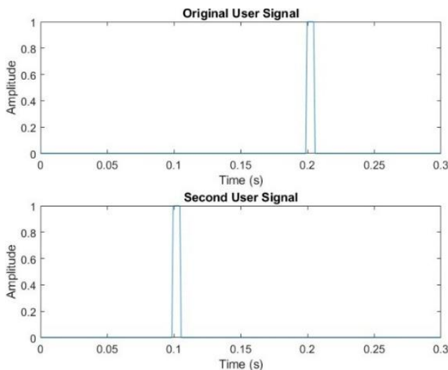
Fig. 3. Time-Domain Signal for Two Users
