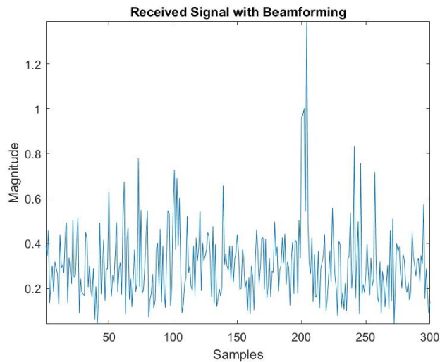
Fig. 10. Received Signal after Beamforming
