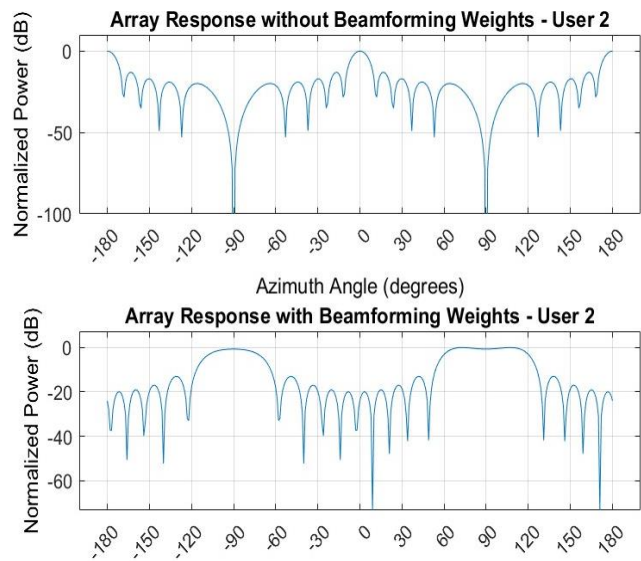
Fig. 12. Azimuth Angles for user2
