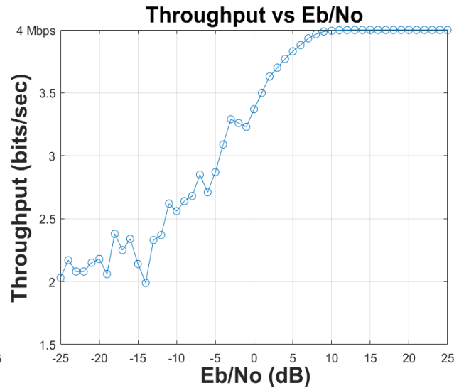
Fig. 14. Throughput vs. Eb/No
